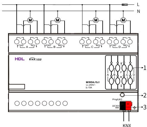
Figure 4. Wiring
