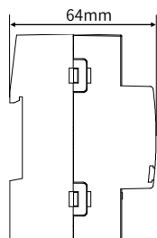
Figure 3. Dimensions - Side View
